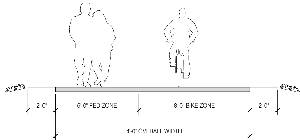
1/4" = 1'-0" Trolley Trail Multiuse Path - After section 01
